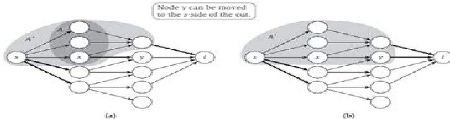
Figure 7.11 (a) A minimum cut in proof of (7.40). (b) The same cut after moving node y to the A' side. The edges crossing the cut are dark.
