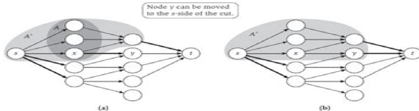
Figure 7.11 (a) A minimum cut in proof of (7.40). (b) The same cut after moving node y to the A' side. The edges crossing the cut are dark.
